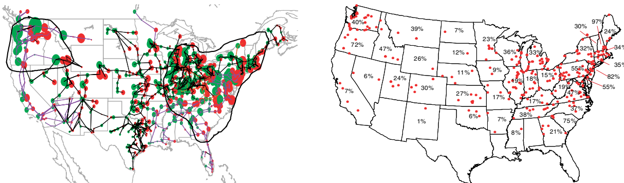
FIGURE C.3 (a; left ) 4800 nT/min geomagnetic field disturbance at 50° geomagnetic latitude scenario. The regions outlined are susceptible to system collapse due to the effects of the GIC disturbance. The region impacted would be of unprecedented scale and involve populations in excess of 130 million. (b; right ) A map showing the at-risk EHV transformer capacity by state for this disturbance scenario. Regions with high percentages could experience long-duration outages that could extend multiple years.
