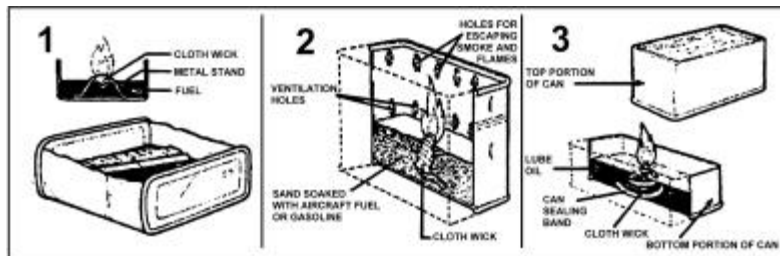
Figure VI-16. Improved Stove
